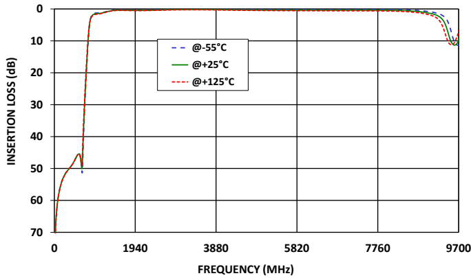
HFCG-880+ INSERTION LOSS
