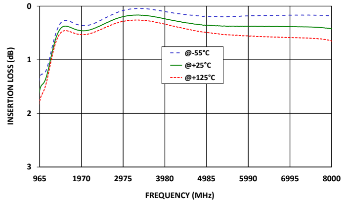
HFCG-880+ INSERTION LOSS (Zoomed)
