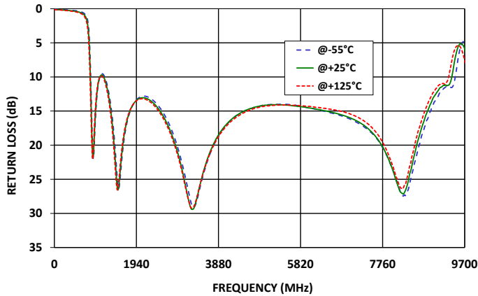
HFCG-880+ RETURN LOSS
