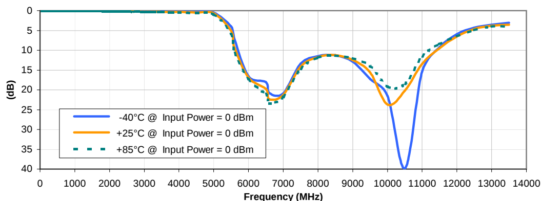
OUTPUT RETURN LOSS vs. TEMPERATURE
