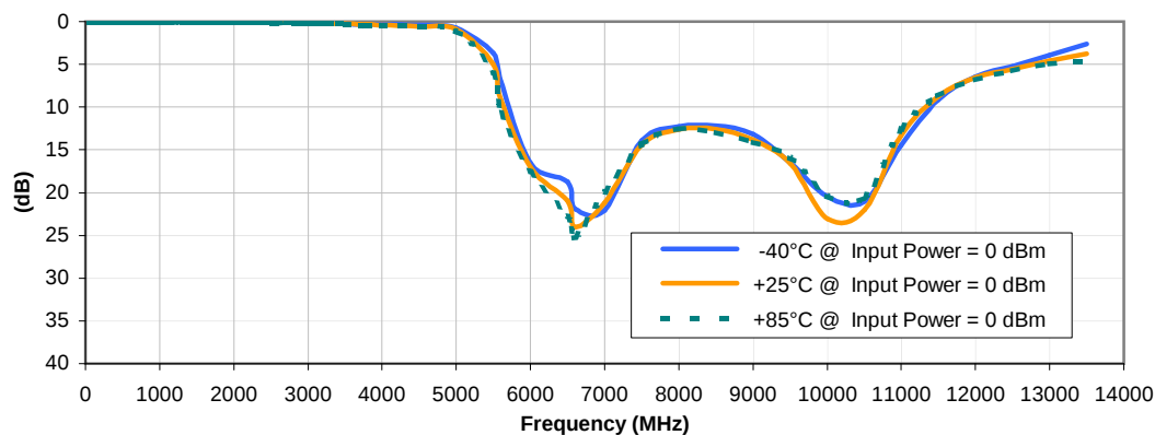
OUTPUT RETURN LOSS vs. TEMPERATURE
