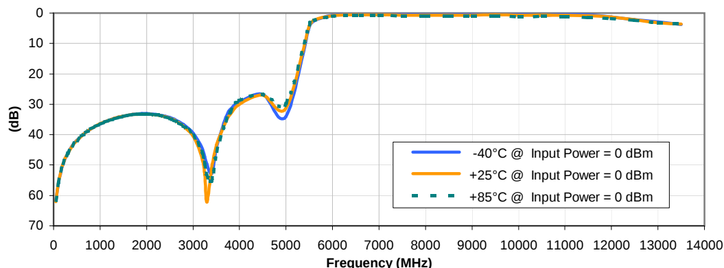
INSERTION LOSS vs. TEMPERATURE
