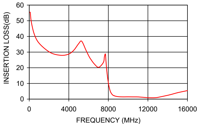
INSERTION LOSS
