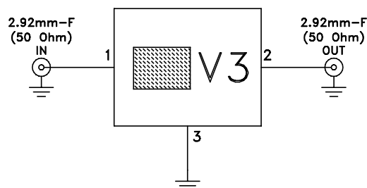
Schematic diagram
