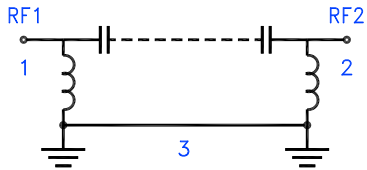
Figure 1. HFHK-3800+ Functional Diagram
