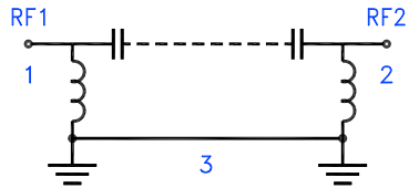
Figure 1. HFHK-4000+ Functional Diagram
