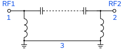
Figure 1. HFHKI-2200+ Functional Diagram
