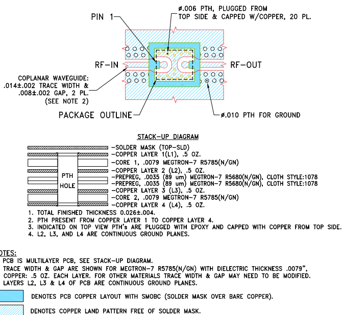
Figure 2. Suggested PCB Layout
