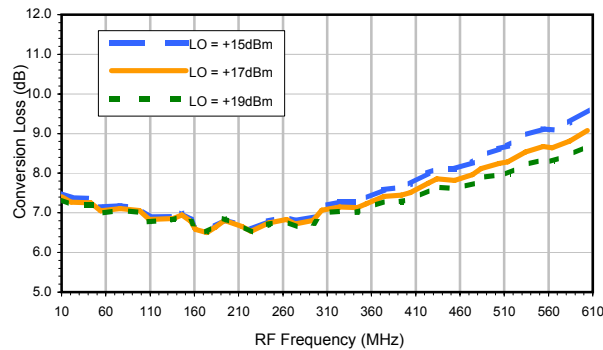
Conversion Loss vs. LO @ RF=155.1 MHz
