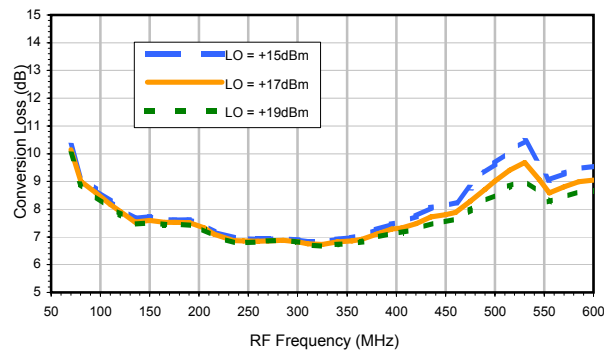
Conversion Loss vs. LO @ RF=310.1 MHz
