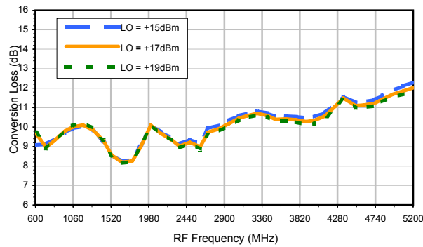
Conversion Loss vs. LO @ RF=2650.1 MHz
