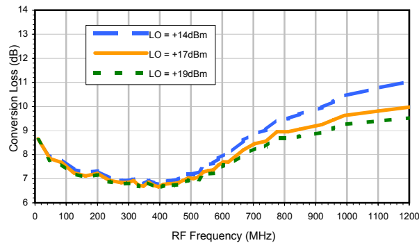
Conversion Loss vs. LO @ RF=620 MHz
