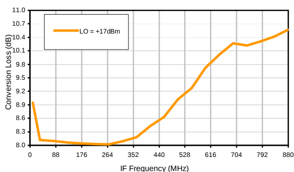
Conversion Loss vs. IF @ RF=2170.1001MHz
