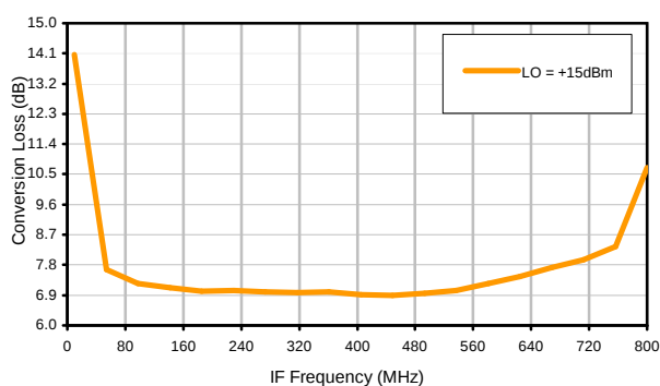
Conversion Loss vs. IF @ RF=3500MHz
