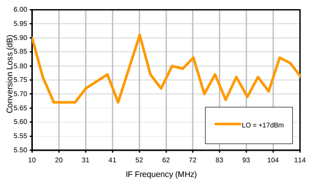
Conversion Loss vs. IF @ RF=137MHz
