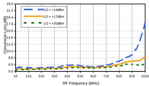
Conversion Loss vs. LO @ RF=124.5MHz
