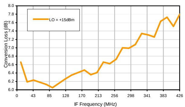
Conversion Loss vs. IF @ RF=458.1MHz
