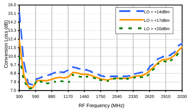
Conversion Loss vs. LO @ RF=2160.1001MHz
