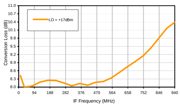
Conversion Loss vs. IF @ RF=2360.1001MHz
