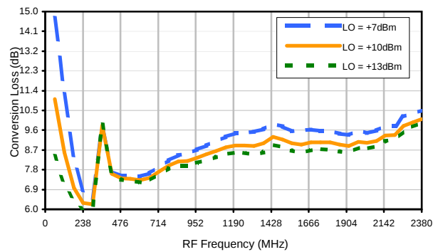
Conversion Loss vs. LO @ RF=621.1MHz
