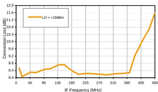
Conversion Loss vs. IF @ RF=2216.1001MHz
