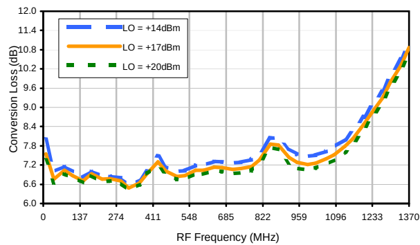
Conversion Loss vs. LO @ RF=238.5MHz
