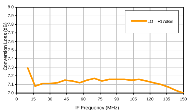
Conversion Loss vs. IF @ RF=180.1MHz
