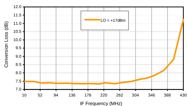
Conversion Loss vs. IF @ RF=1310.1MHz
