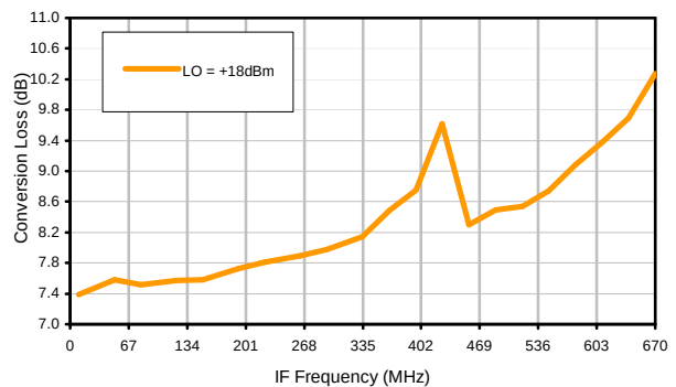
Conversion Loss vs. IF @ RF=909.1MHz
