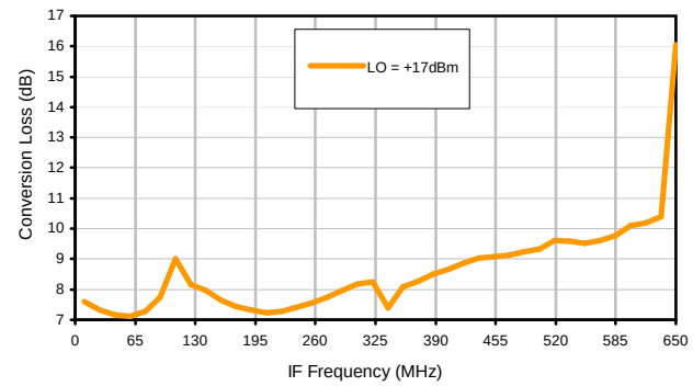
Conversion Loss vs. IF @ RF=660.1MHz
