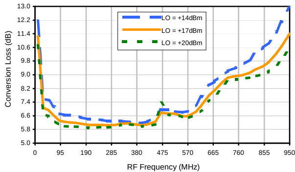
Conversion Loss @ IF=80MHz
