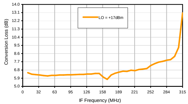
Conversion Loss vs. IF @ RF=325MHz
