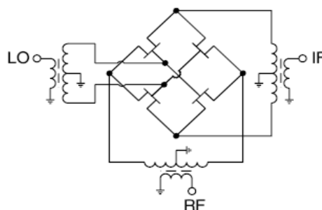
Electrical Schematic
