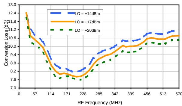
Conversion Loss vs. LO @ RF=170MHz
