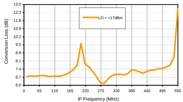
Conversion Loss vs. IF @ RF=560.1MHz
