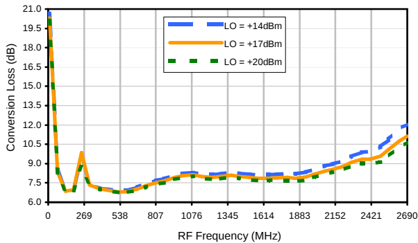
Conversion Loss @ IF=110MHz
