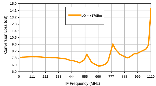
Conversion Loss vs. IF @ RF=1120.1MHz
