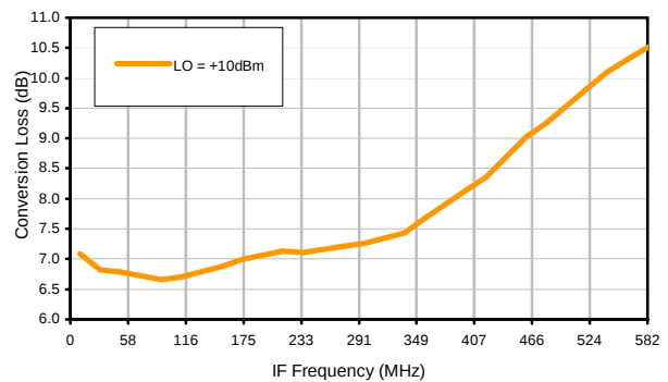
Conversion Loss vs. IF @ RF=1755.1MHz
