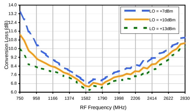
Conversion Loss vs. LO @ RF=1732.5MHz
