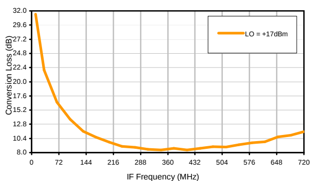
Conversion Loss vs. IF @ RF=2700MHz
