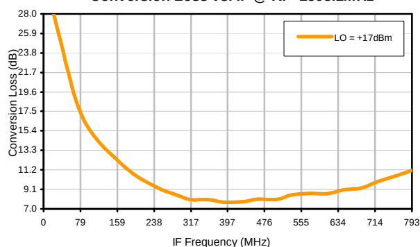
Conversion Loss vs. IF @ RF=2690.1MHz
