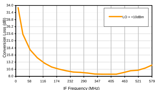
Conversion Loss vs. IF @ RF=3340.1001MHz
