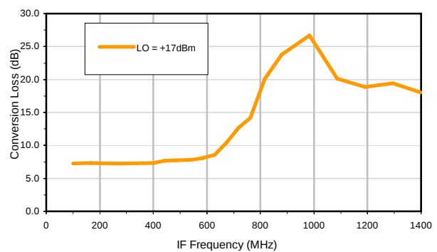
Conversion Loss vs. IF @ RF=1700 MHz
