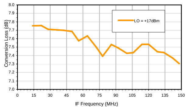
Conversion Loss vs. IF @ RF=170 MHz
