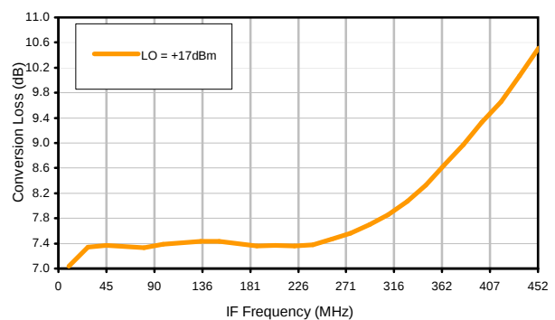
Conversion Loss vs. IF @ RF=1915.1MHz
