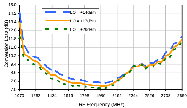
Conversion Loss vs. LO @ RF=1882.5MHz
