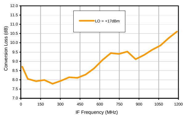
Conversion Loss vs. IF @ RF=1815.1MHz
