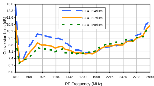
Conversion Loss vs. LO @ RF=1750MHz
