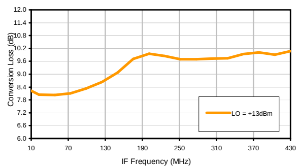
Conversion Loss vs. IF @ RF=1270.1MHz
