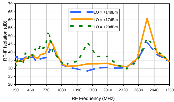
RF-IF Isolation
