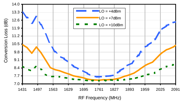
Conversion Loss vs. LO @ RF=1700MHz
