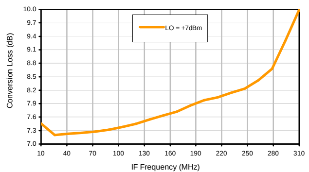
Conversion Loss vs. IF @ RF=1898.1MHz
