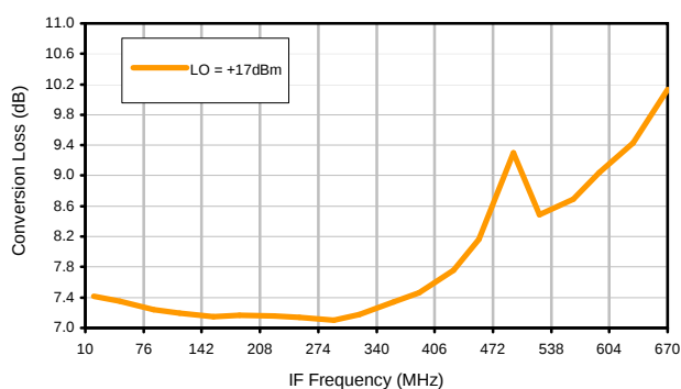
Conversion Loss vs. IF @ RF=1256.1MHz
