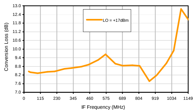
Conversion Loss vs. IF @ RF=3410.1MHz
