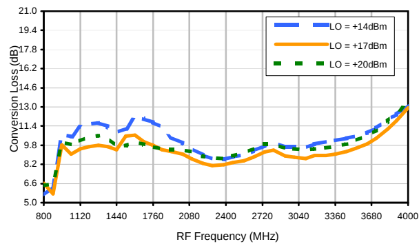
Conversion Loss vs. LO @ RF=2442.1001MHz
