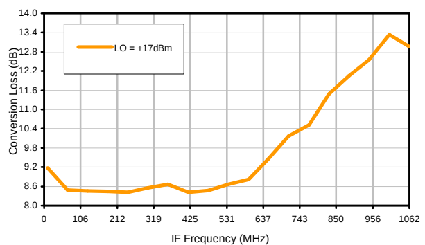
Conversion Loss vs. IF @ RF=2484.1001MHz
