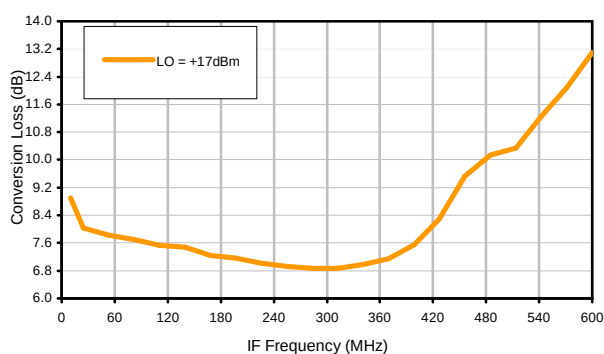
Conversion Loss vs. IF @ RF=928.1MHz
