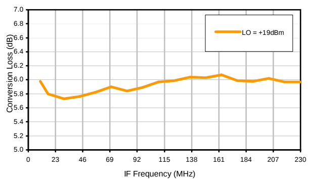
Conversion Loss vs. IF @ RF=340.1MHz
