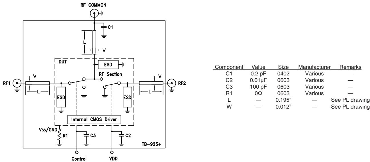
Figure 1. Block Diagram of test Circuit used for characterization (DUT soldered on Mini-Circuit's TB-923+)
