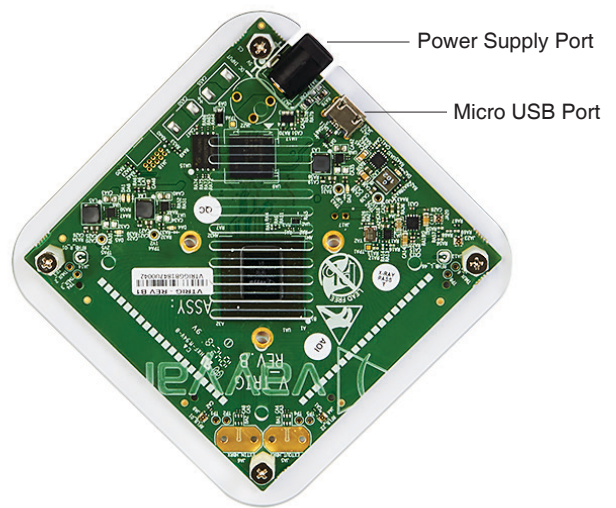
Fig. 5 Front View
