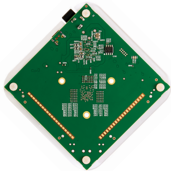
Fig. 3 IMAGEVK-74 RF Sensor Unit PCB Bottom View
