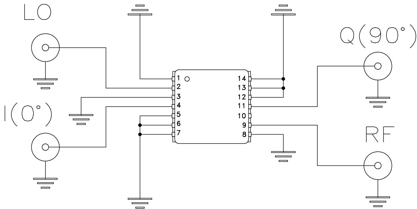
Schematic Diagram
