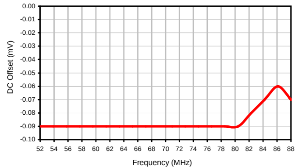
DC Offset
