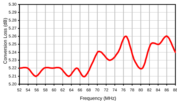
Conversion Loss
