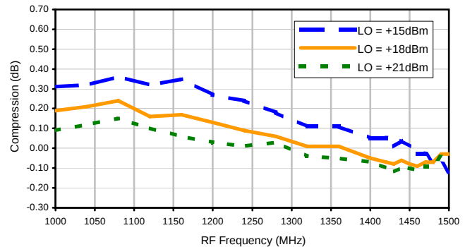
COMPRESSION @ RF=+11dBm
