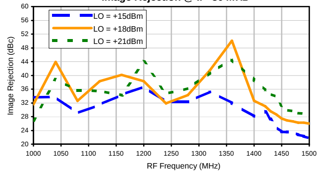
Image Rejection @ IF=80 MHz
