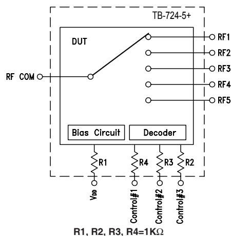
Figure 1: Block Diagram Of Test Circuit Used For Characterization. (DUT soldered on Mini-Circuits' TB-724-5+)
