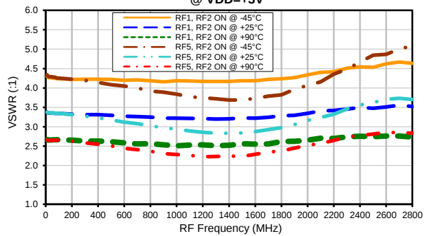
VSWR vs. Frequency & Temperature; RF1 & RF5 (OFF) @ VDD=+3V
