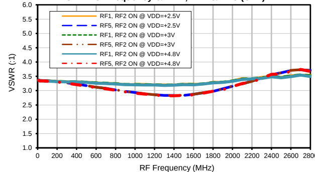
VSWR vs. Frequency & VDD; RF1 & RF5 (OFF)
