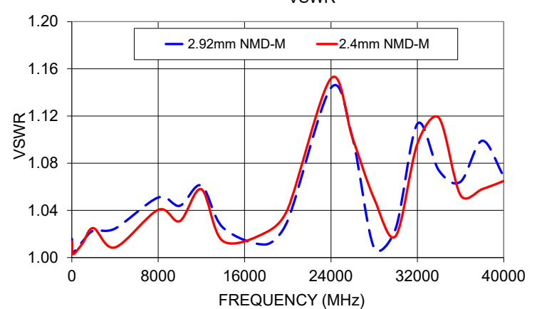
KMNMMD-24MNMMD+ VSWR
